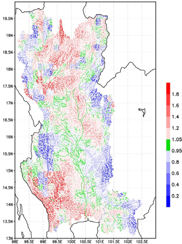
Fig. 9 Change of the ratio of the 10-years return period river discharge in the future climate experiment with respect to the present climate experiment.
