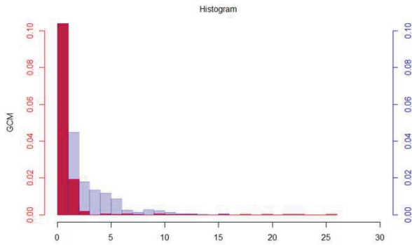
Fig. 7 Histogram of runoff generation data in GCM outputs and reference data in July for 20 years
